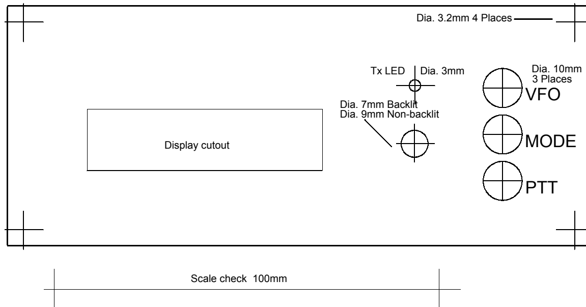
Controller drilling template
